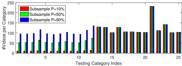
Fig. 9 Distribution of testing videos after subsampling.
