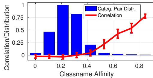
Fig. 6 The connection between transfer efficacy and class-name affinity: Illustrated by class correlation v.s. class name affinity.
