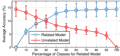
(a) Maximal class name affinity
