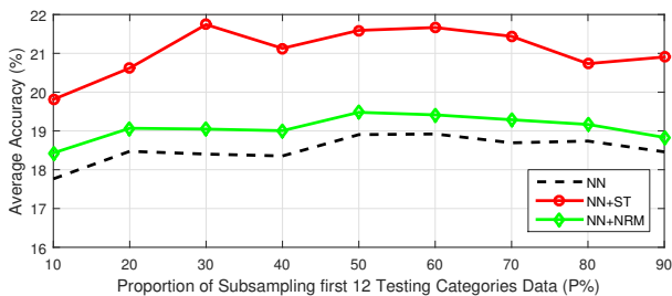
Fig. 10 Performance of ZSL for subsampled imbalanced test set.
